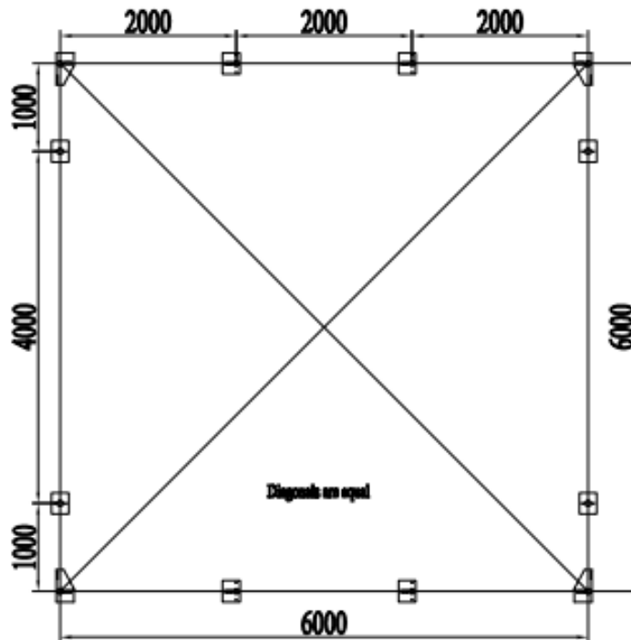
Figure 3 Position of Base Flanges
