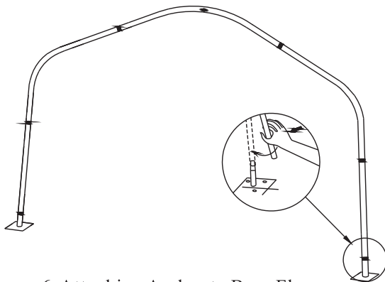
Figure 6 Attaching Arches to Base Flanges
