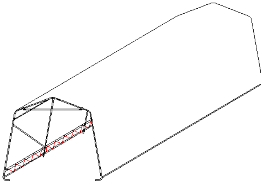
Figure 6 Fastening the Roof Cover
