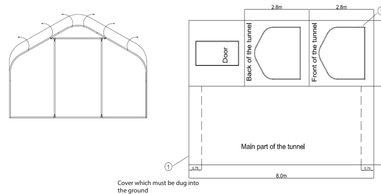
Cover hobby tunnel 2,0x2,0xL [m]
