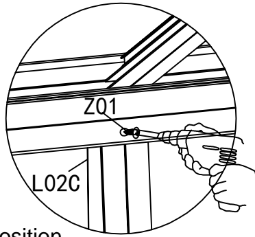
Screw position
