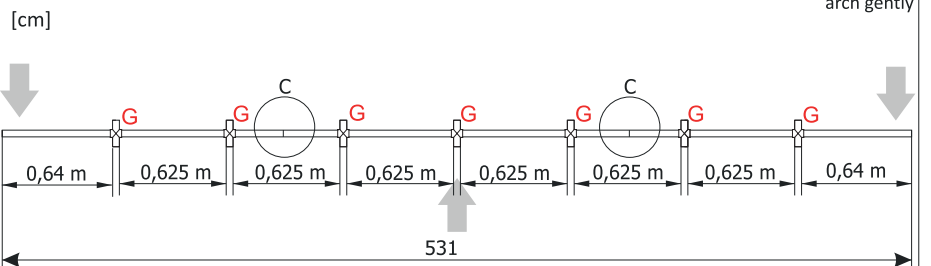
Scheme 2b middle bows (16 pcs)
